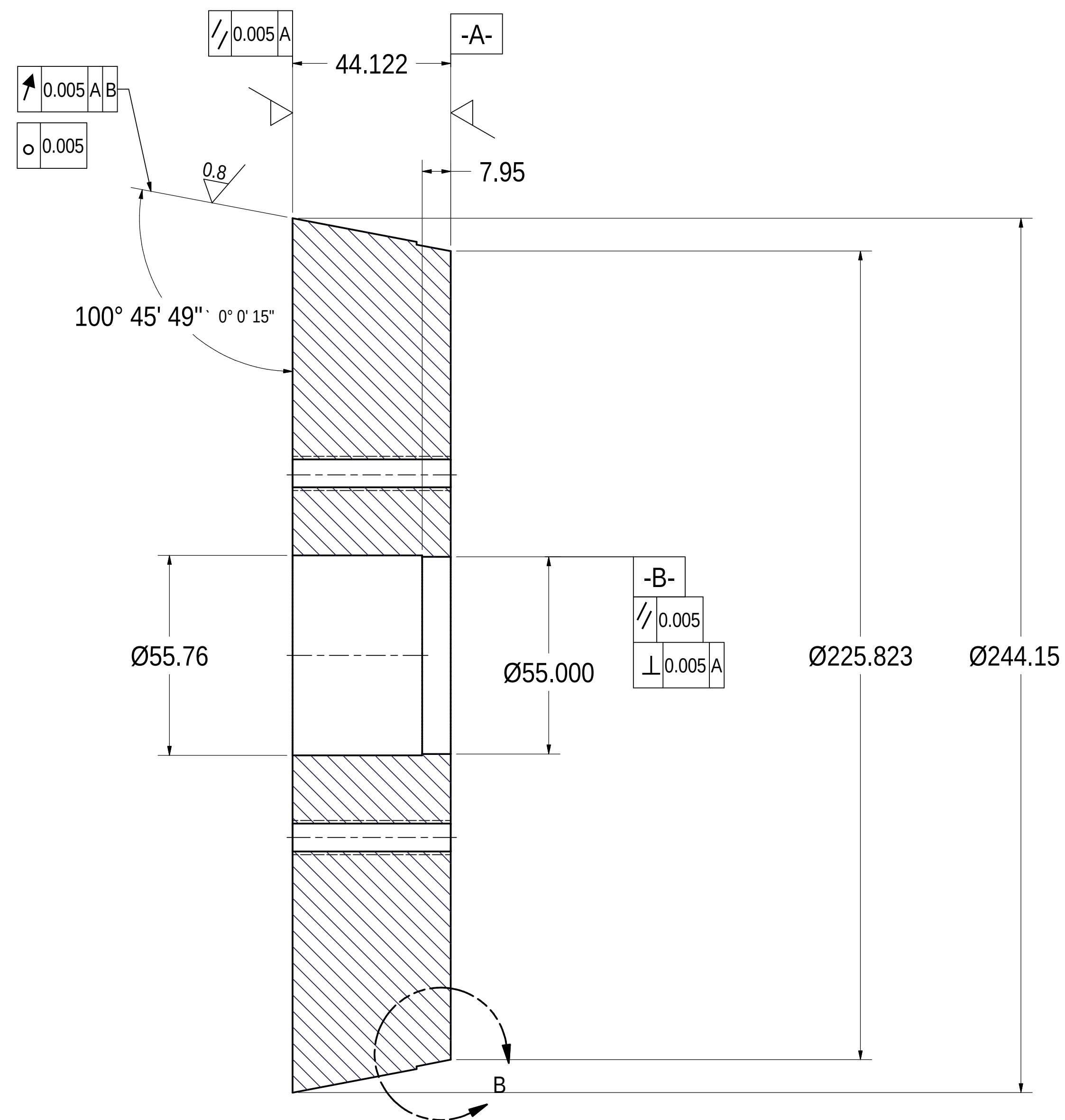
SECTION E-E SCALE 1:1
